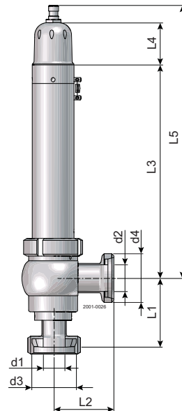
Standard DN25 with inductive sensor for feedback
