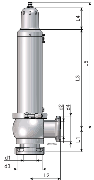
Standard DN40-DN100 with inductive sensor for feedback
